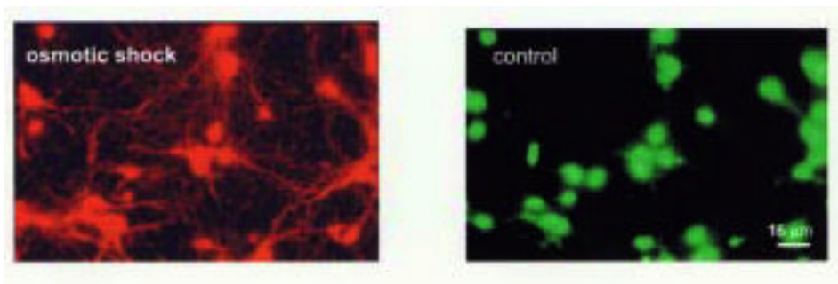
Figure 5. Stress evoked by osmotic shock changes the intracellular localization of the splicing regulatory proteins htra2- 1. Cells were subject to 3 hours of hyperosmotic medium and then stained for htra2- 1 (left). When compared to untreated cells, a translocation of splicing regulatory proteins is apparent.
