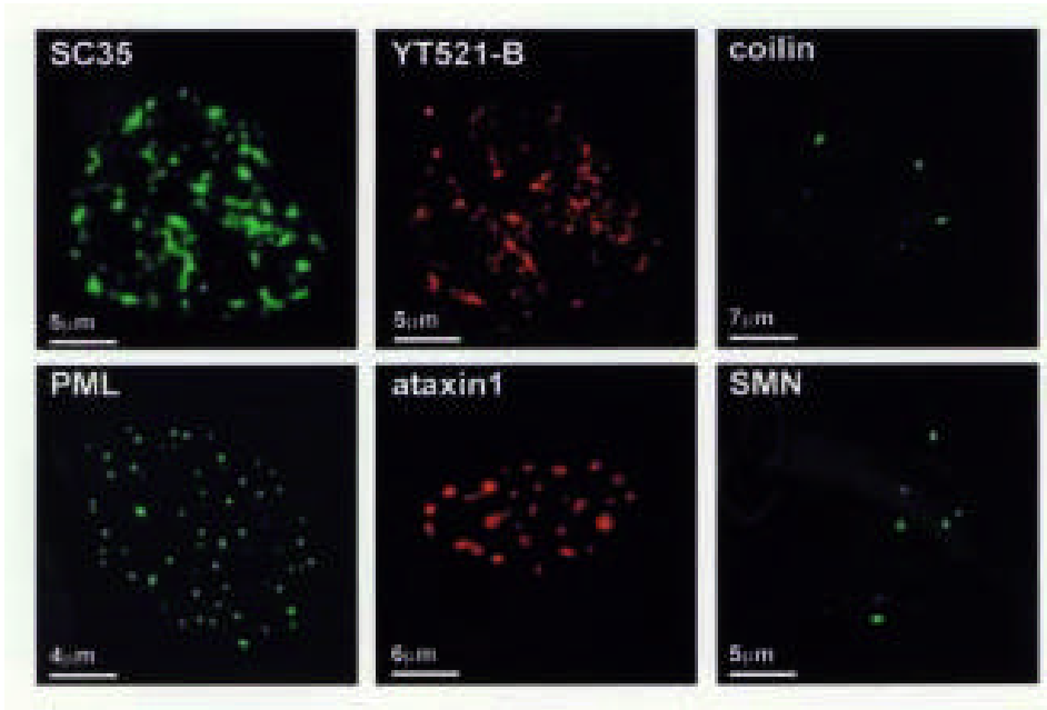
Figure 4. Subnuclear compartments visualized with endogenous antibodies of as GFP-fusion proteins (ataxin-1) Subnuclear compartments include SC35-speckles (Fu and Maniatis, 1992) YTBodies containing YT521-B (Nayler et al, 2000) coiled bodies (Carmo-Fonseca et al, 1992) containing coilin, PML bodies (Grande et al, 1996) nuclear inclusion, such as the ones formed by ataxin-1 (Skinner et al, 1997) and gems (Liu and Dreyfuss, 1996) formed by SMN (survival of motoneuron).
