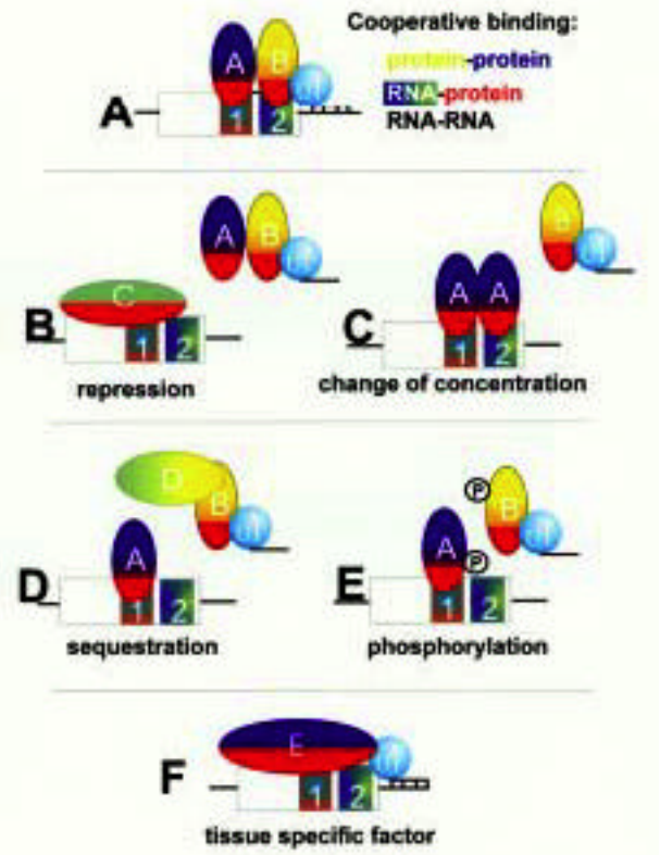
Figure 3. Model for alternative splice site regulation (A) An exon (box) is recognized by binding of multiple proteins (A, B) on splicing enhancers located on the pre-mRNA (t, 2). Splicing of this exon is initiated by contact with components of the constitutive splicing machinery, shown here as the U1 snRNP (U1). The formation of this complex is cooperative and involves protein:protein interactions, RNA:protein interaction and RNA: RNA interactions that are indicated by different colors. This complex can be regulated by several ways: (B) A protein C with higher affinity to the enhancer sequences can repress the exon usage by competing with proteins A and B for binding to the exon. (C) The recognition is concentration dependent, as an increase of the concentration of protein A could compete for binding with protein B. (D) Likewise protein B could be sequestered by a different protein D (E) Phosphorylation can influence the binding of individual factors assembling around exon enhancers (F) Tissue specific factors can recognize a protein in a cell type or tissue specific way.
