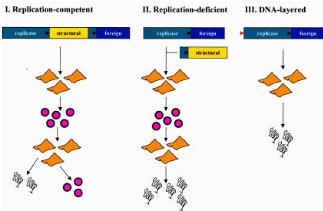
Figure 1. Schematic presentation of alphavirus expression systems., \blacktriangle , 26S subgenomic promoter; \blacktriangleright , CMV promoter; \diamond , mammalian host cell; \bullet , alphavirus particle; \text{⌘} , recombinant protein
